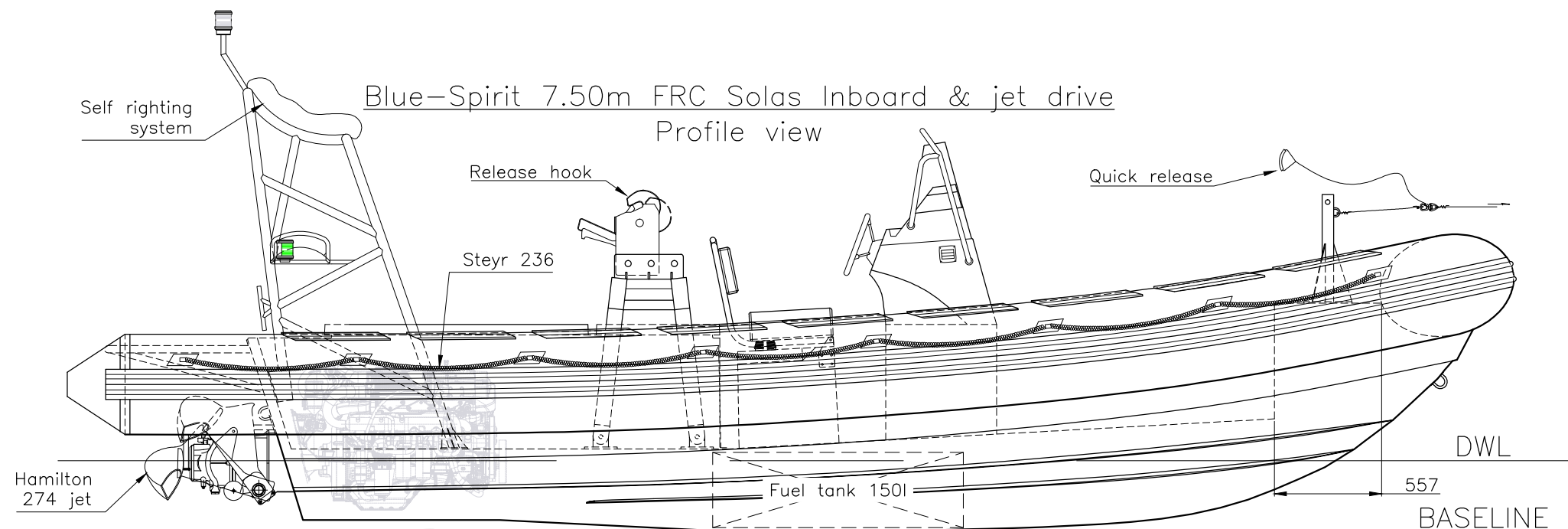
Blue Spirit 7m50 FRC Solas
