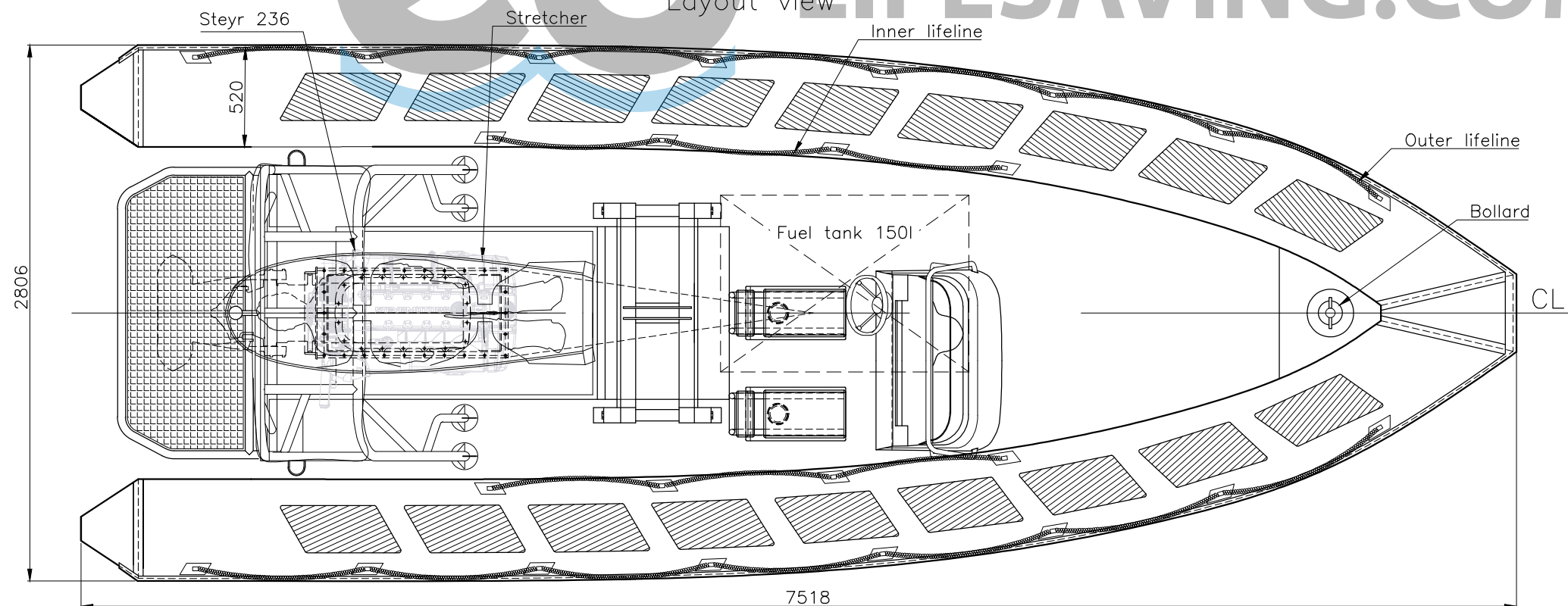
Blue-Spirit 7.50m FRC Solas Inboard & Jet drive Layout view
