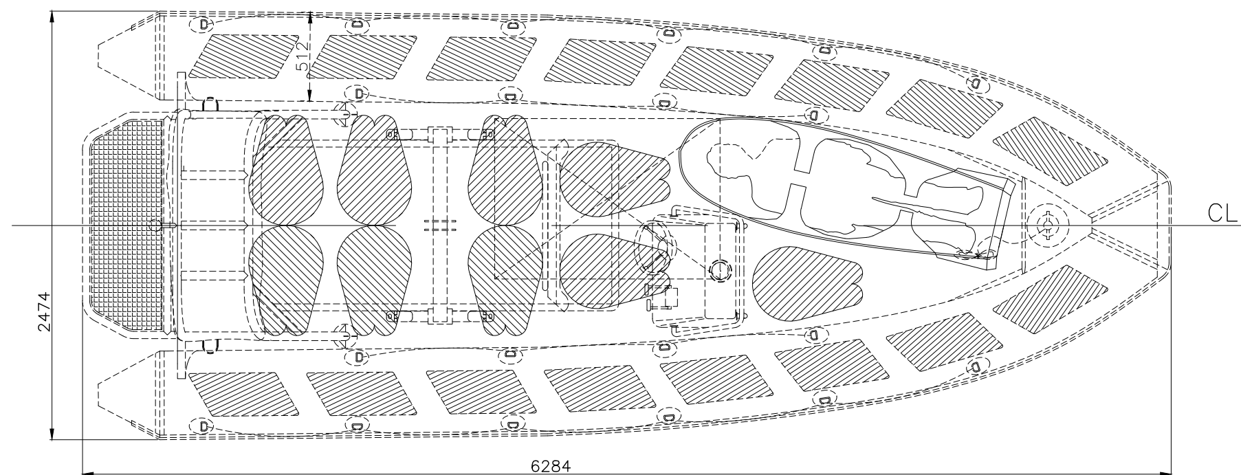
Blue-Spirit 6.20m FRC Solas Inboard & sterndrive Layout view
